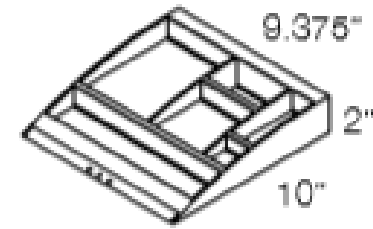
Accessories Tray
