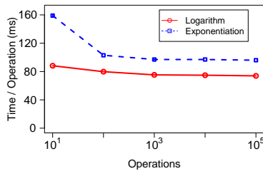
Fig. 2. Performance of floating point exponentiation and logarithm.
