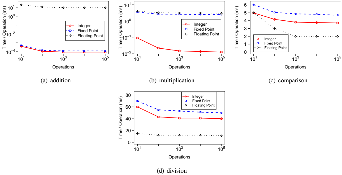
Fig. 1. Performance of basic operations for different data types.
